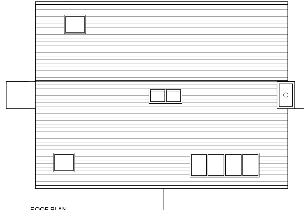
ROOF PLAN
