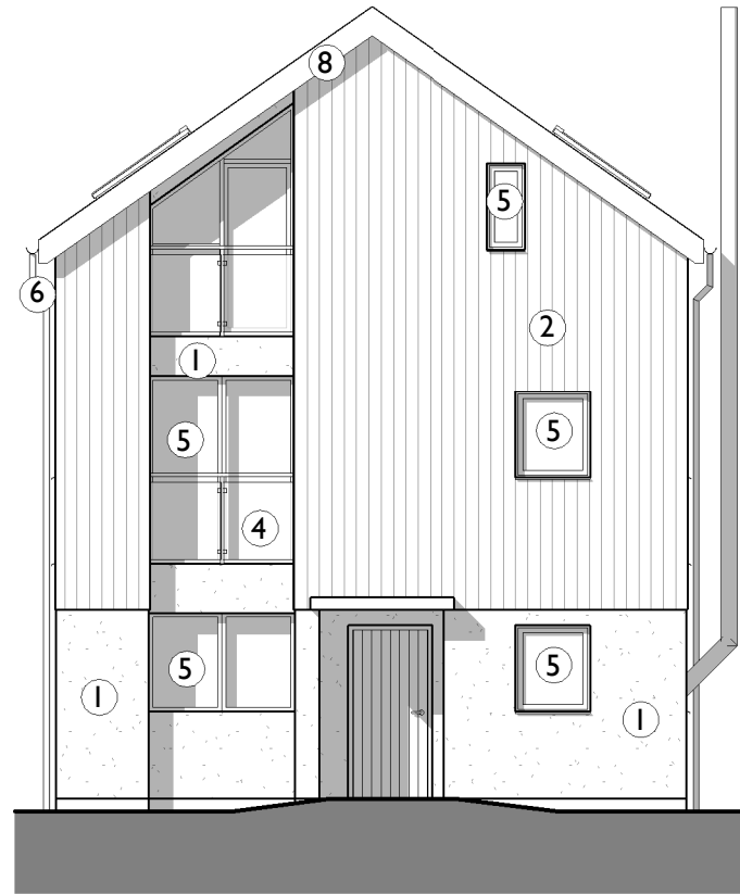
FRONT ELEVATION
