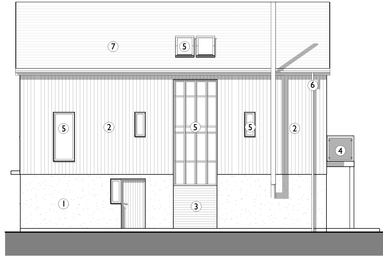
SIDE ELEVATION
