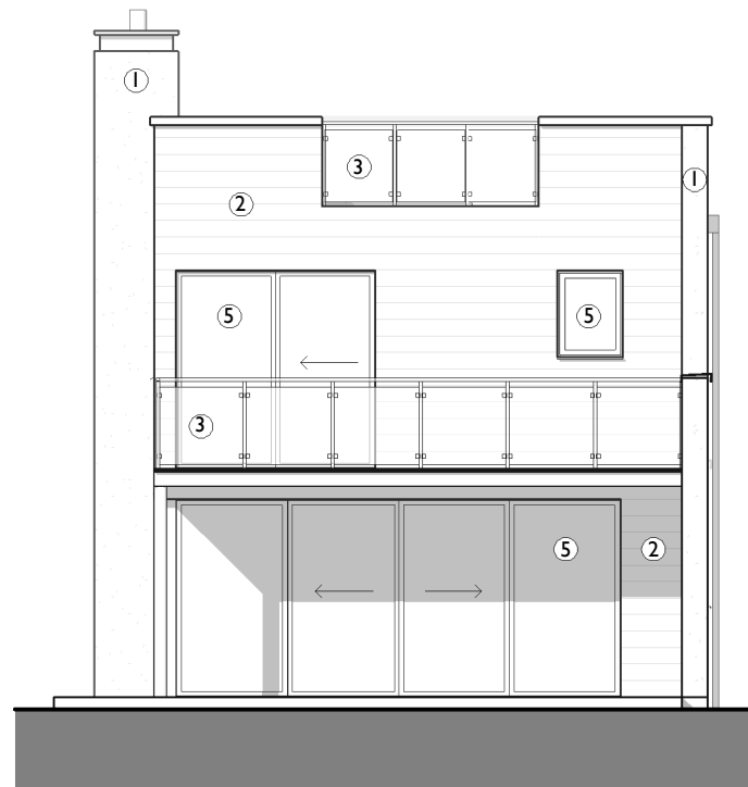
REAR ELEVATION
